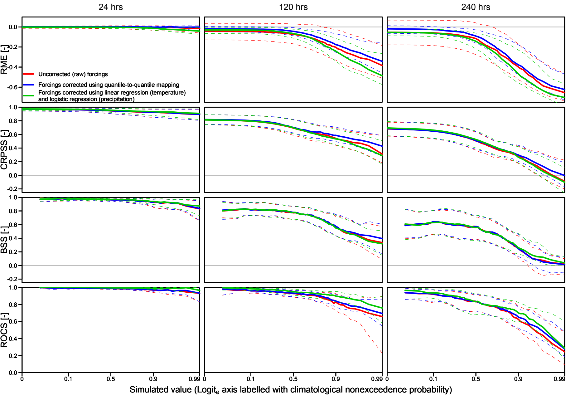
RME, CRPSS, BSS and ROCS for ensemble streamflow forecasts for the 43 headwater basins at 24-hour, 120-hour and 240-hour lead times. For CRPSS, BSS and ROCS, the baseline is formed by sample climatology.
